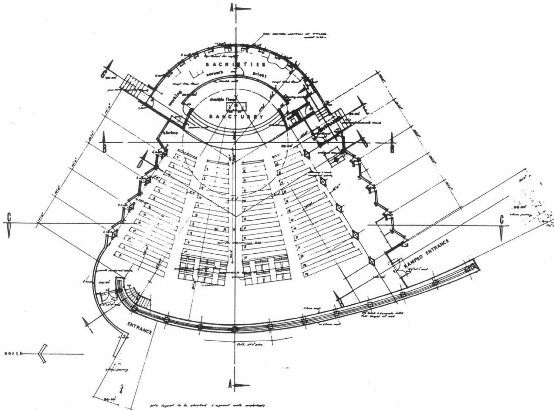
Working drawing, Plan
